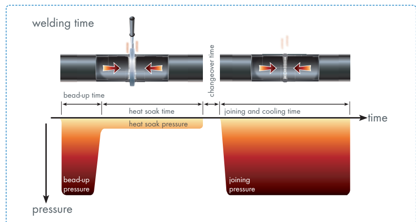
Fig 1-9: Time flow for butt fusion welding in accordance with DVS 2207 Part 1
