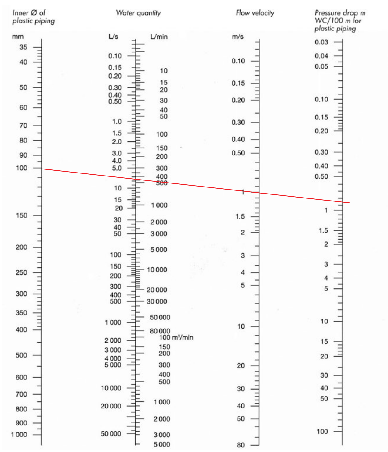
Fig 2-28 — = Example: An inner diameter of 100 mm and a flow velocity of 1 m/s results in a volume flow of 450 l/min and a pressure drop of approx. 0.85 mWC/100 m (0.085 bar)
