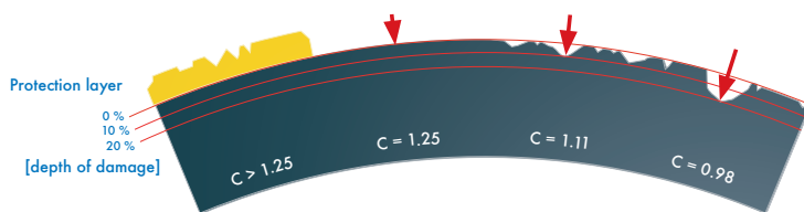
Fig 2-18: Consideration of the safety factor C in relation to score depth
