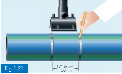
Fig 1-21 Marking the area from which the outer layer is to be peeled
