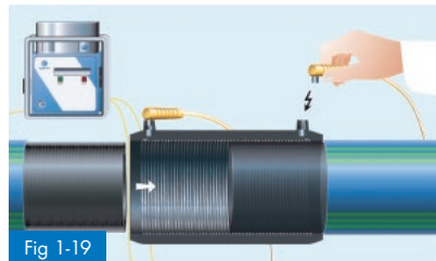
Fig 1-19 Welding procedure acc. to DVS 2207, Part 1
