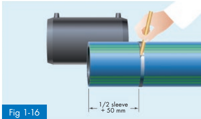
Fig 1-16 Marking the area from which the layer is to be peeled
