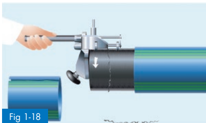
Fig 1-18 Removal of the oxide layer using a rotary scraper
